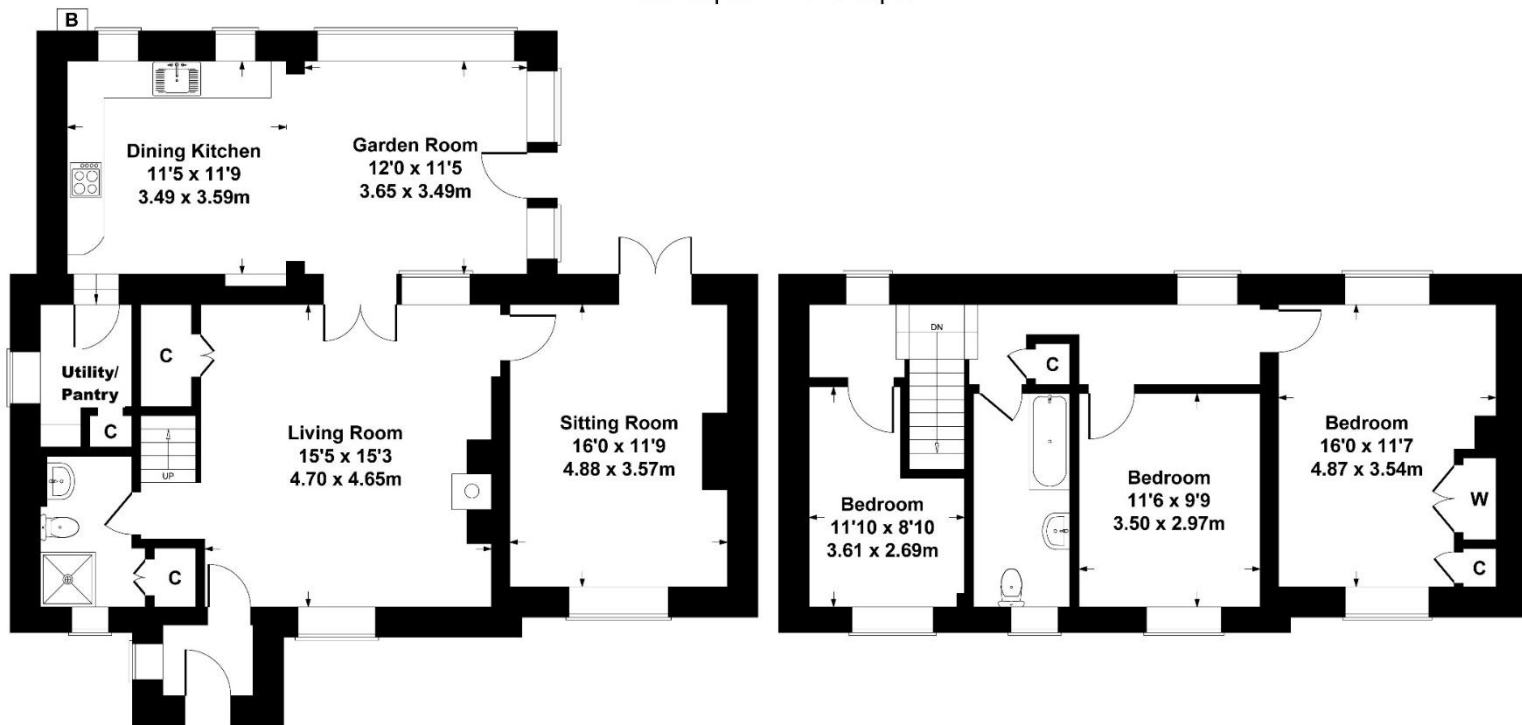
GROUND FLOOR
